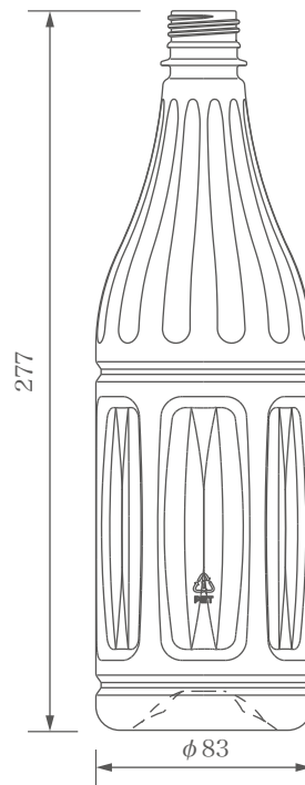
FBHI-900
