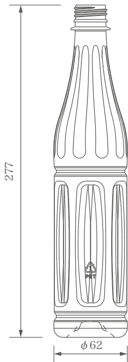
FBHI-500
