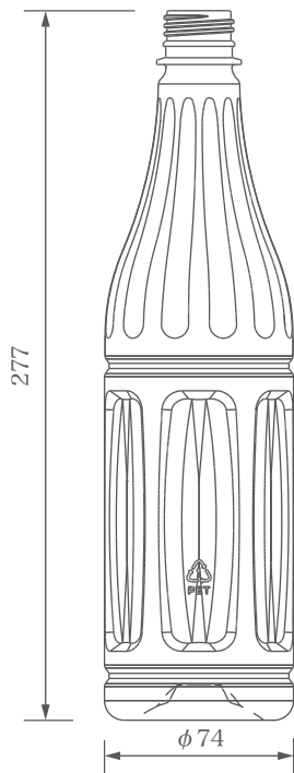
FBHI-720
