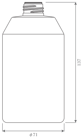
PMP-400(25.0G) Weight: 25g (24% lighter than existing product)
