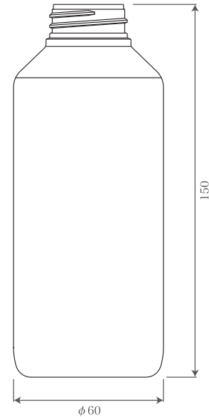
PMP-330IIA(30.5G) Weight: 30.5g (30% lighter than existing product)
