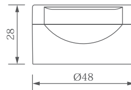
T-50φ M Flip-Top Cap (Textured)
