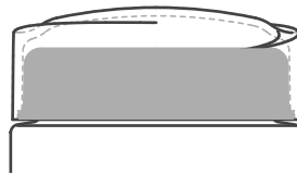
C-70 EO Cap II Material: PP [Inner] / PET [Outer]
